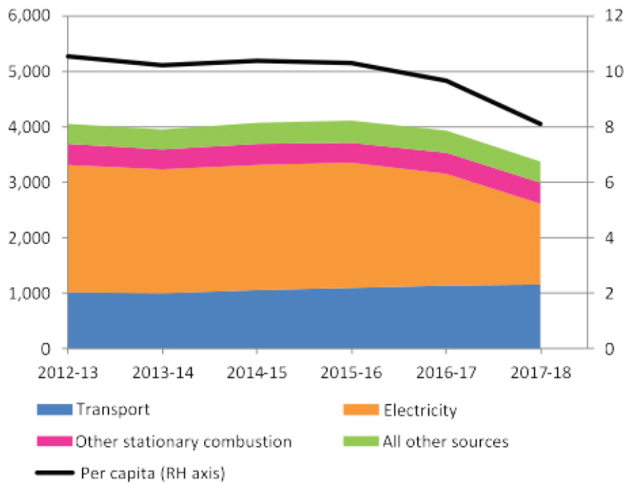
Figure 1: Emission trends in the ACT since 2012-13
