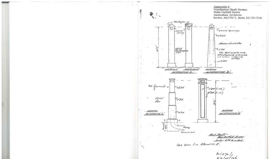
Brownless' Design for the Main Outfall Sewer Ventilation Shafts Credit: Hore, 1994
