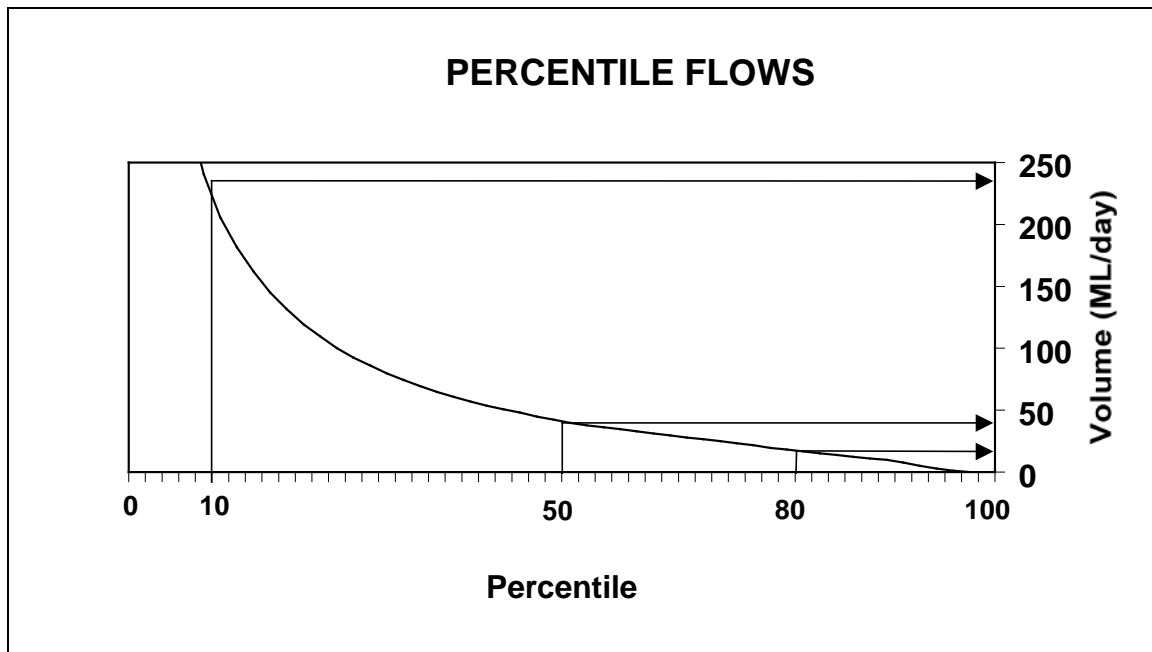
Figure 2: A graphical representation of percentile flows
